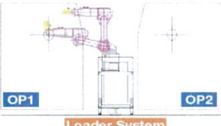
Loader System For 2 units of CNC Lathe machine
